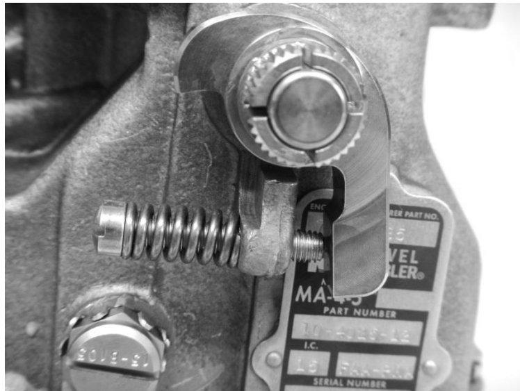
Figure 5-6a: Idle Position
