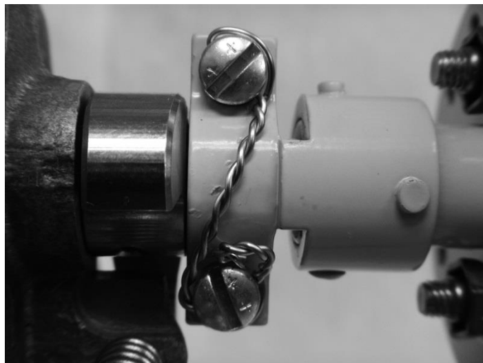
Figure 5-6c: Safety Wiring of Throttle Linkage Adapter Screws
